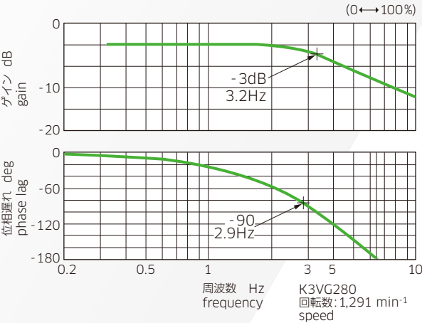
◆周波数応答 Response in the frequency domain
