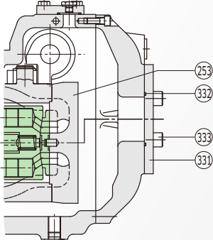
〔吸入弁付回路用(400型)〕 for semi-closed circuit
