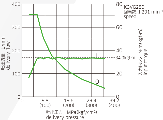
◆馬力制御特性 Horsepower control characteristics
