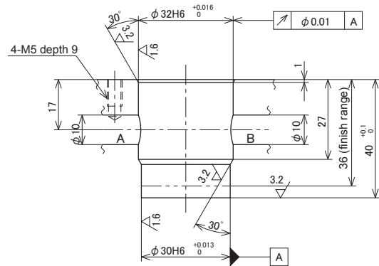
Machining dimension of manifold
