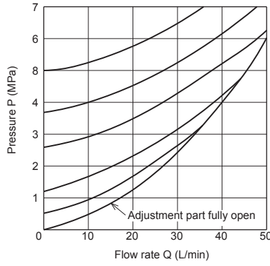
●RD6/315
