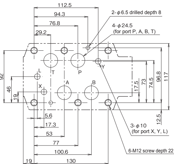
Machining dimension of manifold
