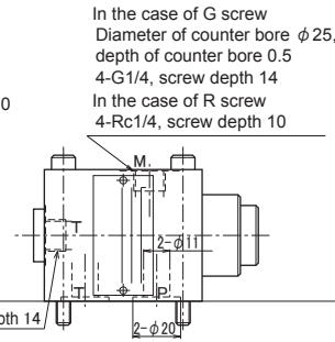
Gasket connection type (Same as G screw connection type other than dimensions entered)
