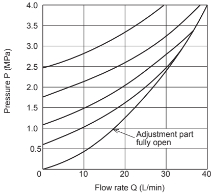
●RD6/200
