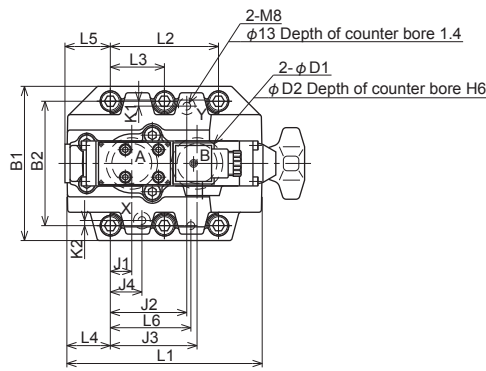
● Handle adjusting type
