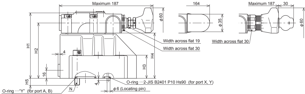
● Screw adjusting type
