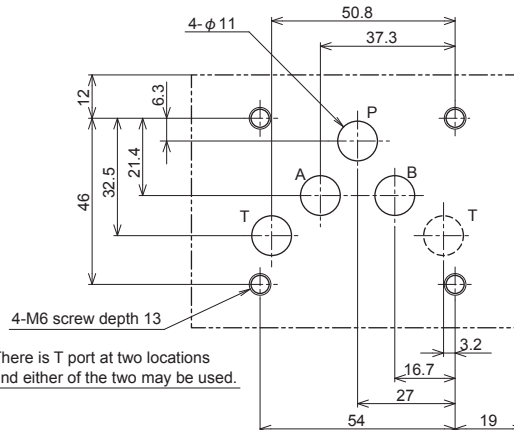
Machining dimension of manifold
