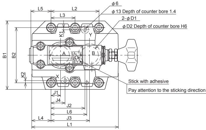
● Handle adjusting type
