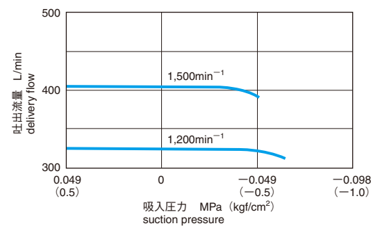
◆吸入能力 / Self-priming capability
