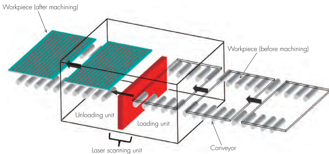
Fig. 1 System configuration
